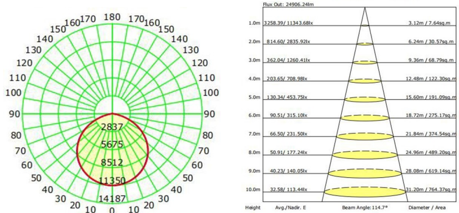
PHOTOMETRY
