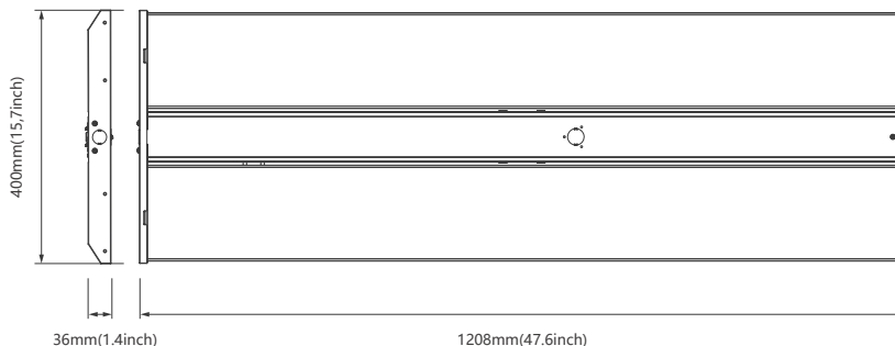
H6-160/220/320W-XY-Z
