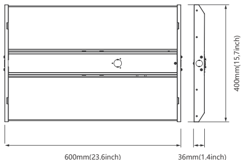
H5-160/220/320W-XY-Z
