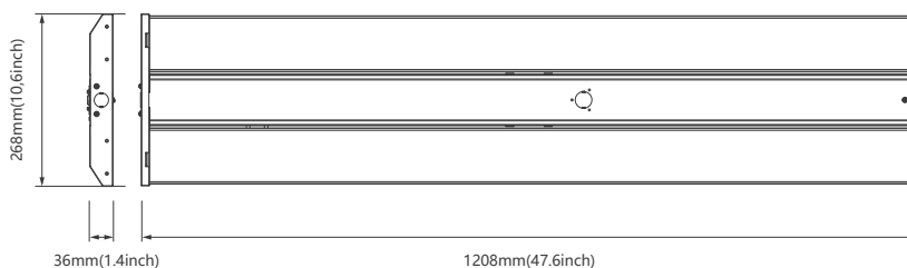
H3-100/160/220W-XY-Z
