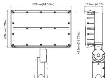
135W&200W(Slipfitter Mount)
