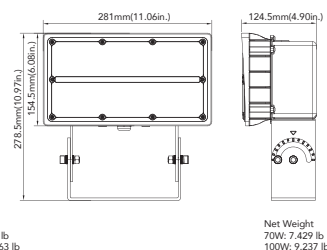
70W&100W(Yoke Mount)
