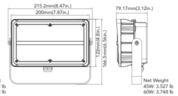
45W&60W(Trunnion Mount)
