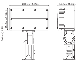
250W/350W(Trunnion Mount)
