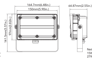
15W&27W(Trunnion Mount)
